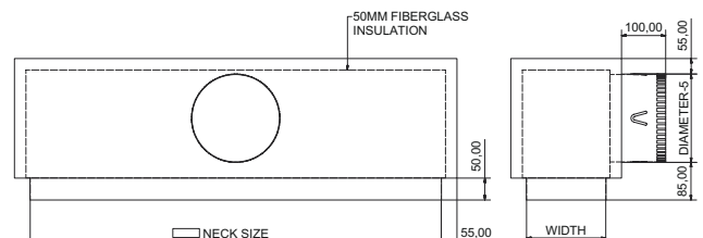
MODEL INSPB-50F (Insulated Plenum Box - 50mm Fibreglass)
