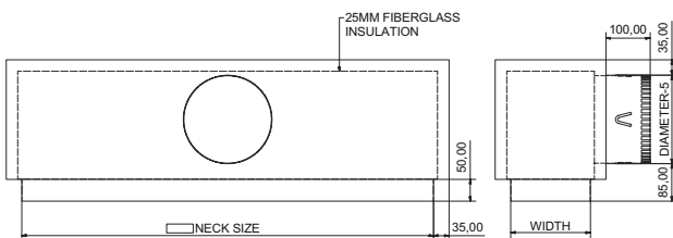
MODEL INSPB-25F (Insulated Plenum Box - 25mm Fibreglass)
