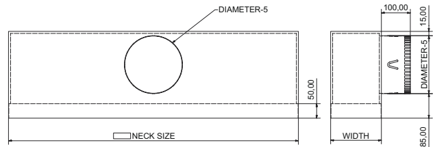
MODEL INSPB-6 (Insulated Plenum Box - 6mm Foam)
