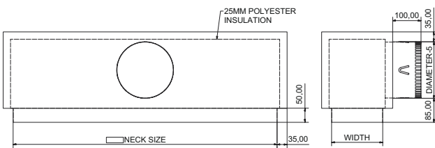
MODEL INSPB-25P (Insulated Plenum Box - 25mm Polyester)
