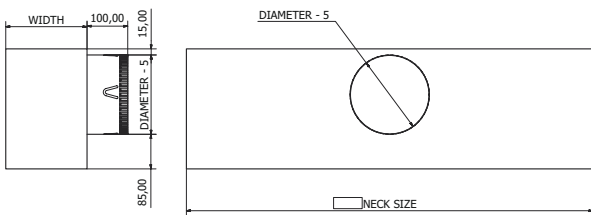
MODEL PPBX (Plain Plenum Box)
