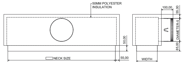
MODEL INSPB-50P (Insulated Plenum Box - 50mm Polyester)
